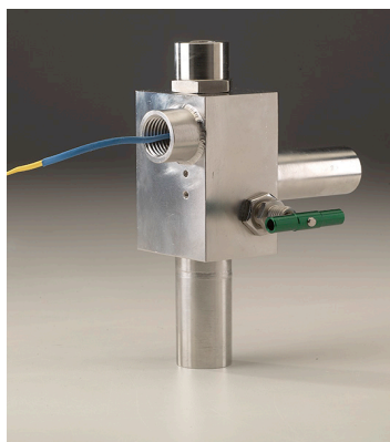
Ultra High Purity Excess Flow Valves, Manual Reset Series, shown here customized with 1/2" welded tube stubs
